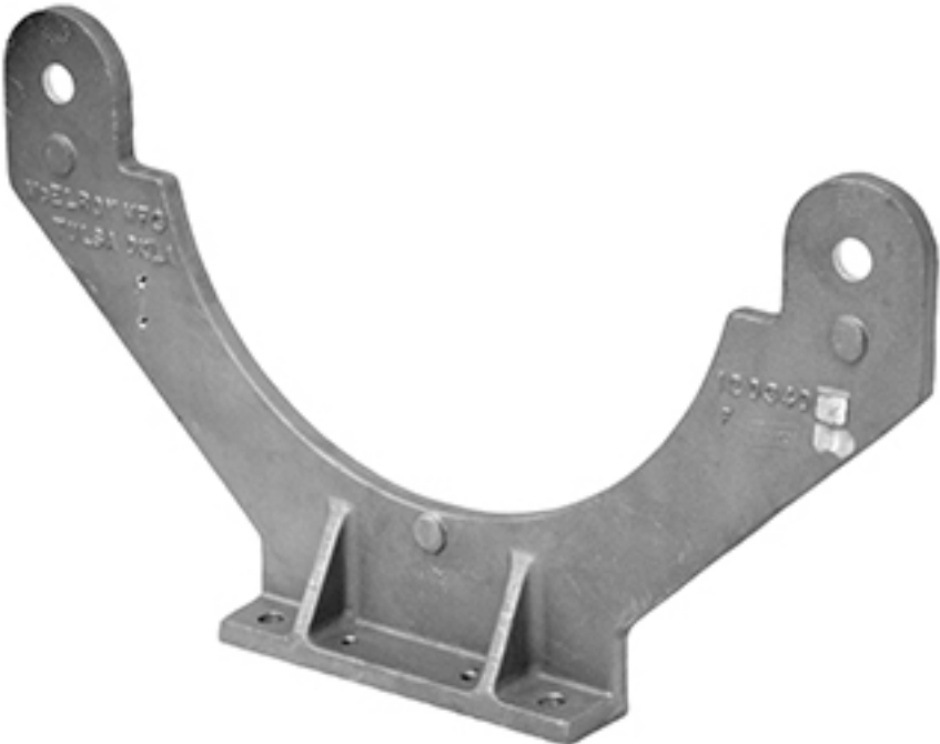
Guide rod support plate
