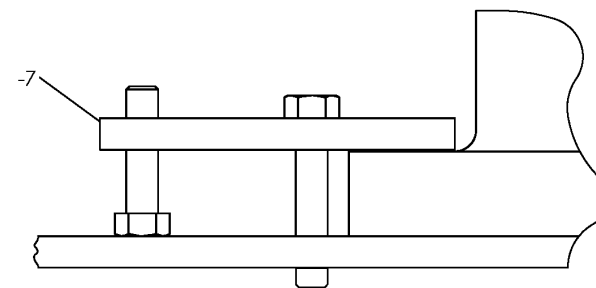
TYPICAL CLAMPING DETAIL USING A4812608 CLAMP KIT
