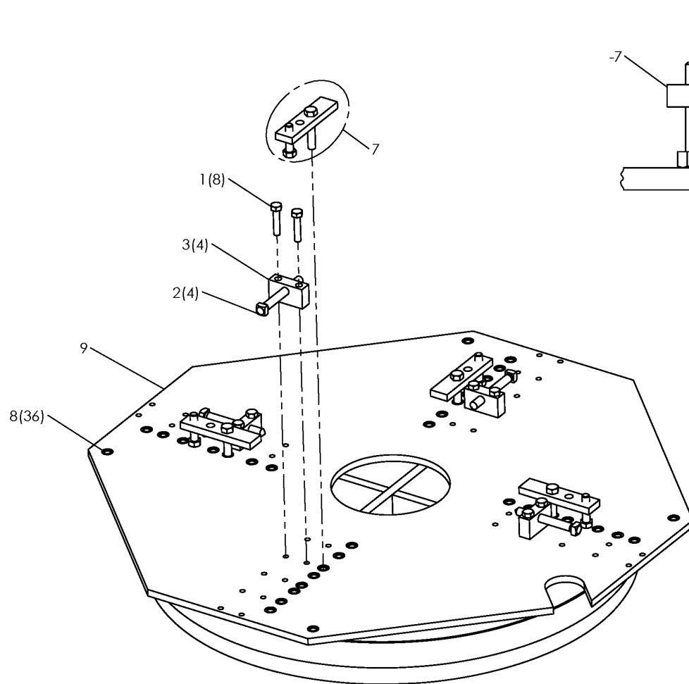
TYPICAL CLAMPING DETAIL USING A4812608 CLAMP KIT
