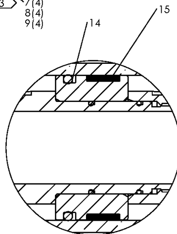
DETAIL B
