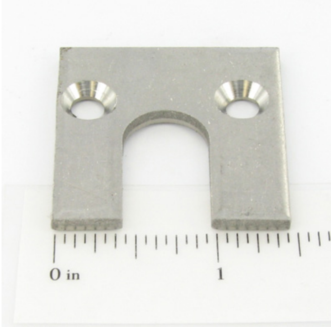
Clamp pad
