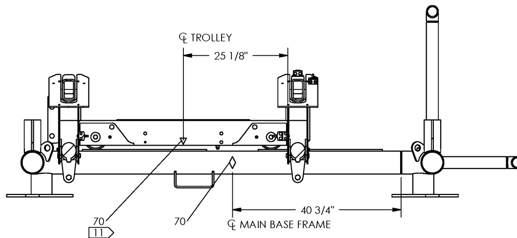
SECTION G-G
