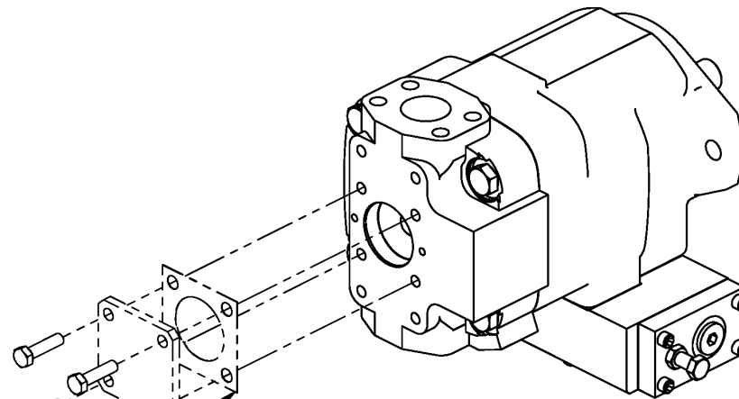
DETAIL A ROTATED (SHOWING MODIFICATION)
