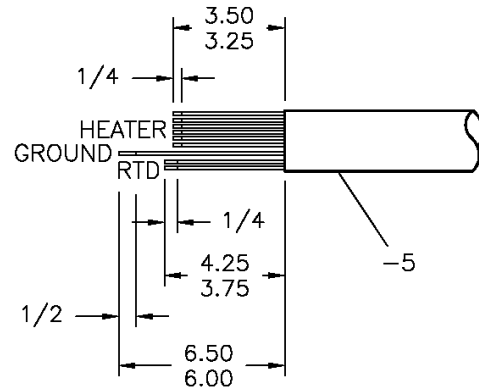
LEAD CUT LENGTH DETAIL
