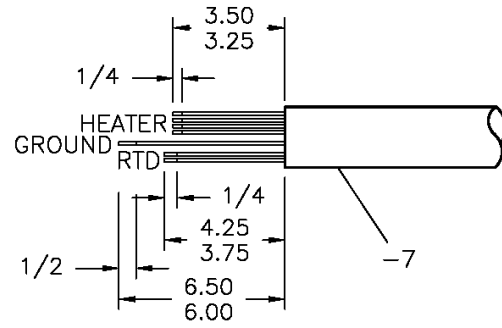
LEAD CUT LENGTH DETAIL
