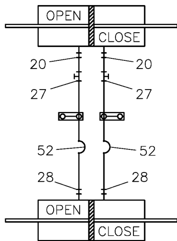
RIGHT CARRIAGE CYLINDER (OPERATOR'S SIDE)
