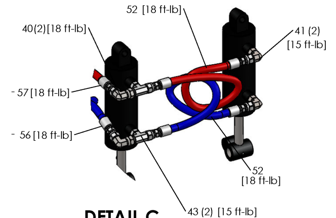
DETAIL C
