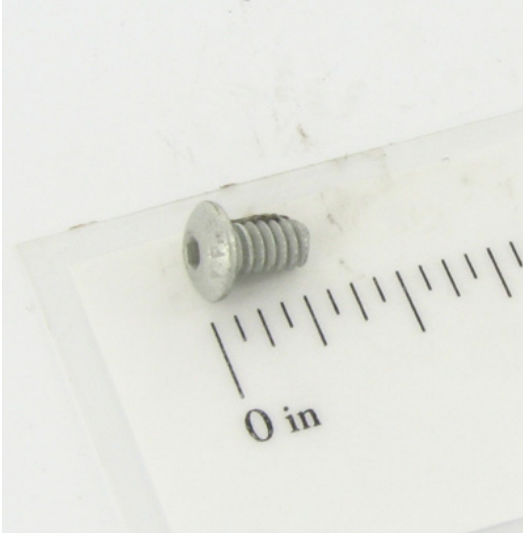
#6-32ncx1/4lg bhscs
