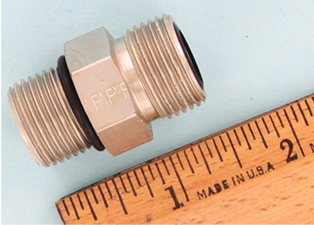
8msl/8msae adapter
