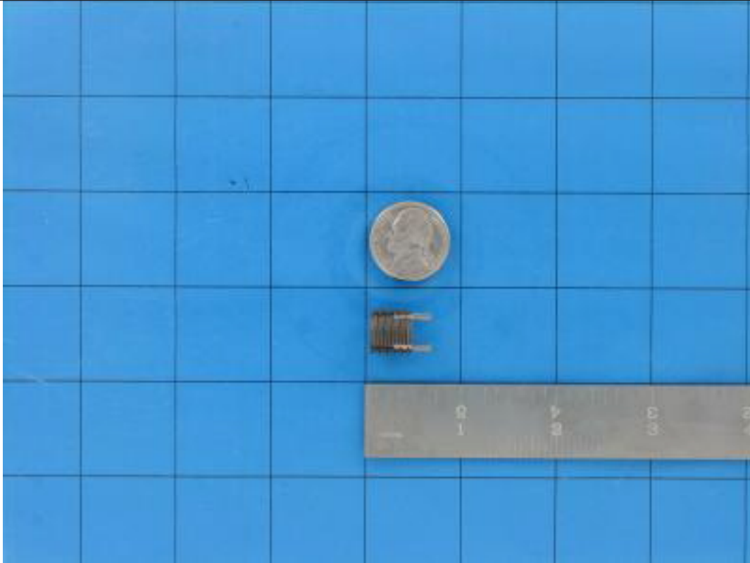
Keensert 5/16-18
