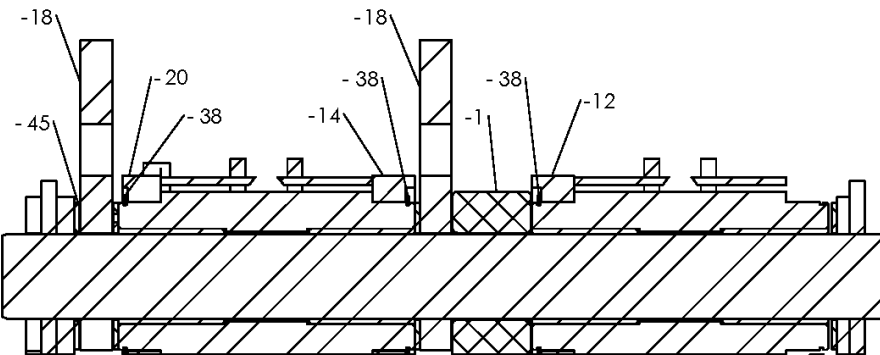
SECTION G-G
