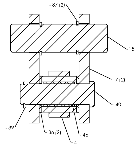
SECTION H-H
