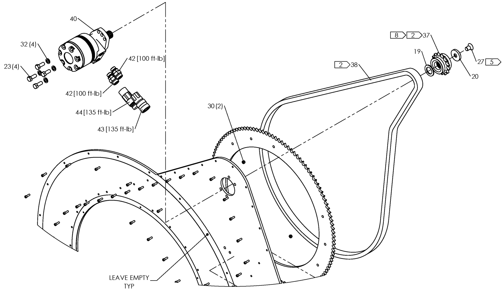
DETAIL A
