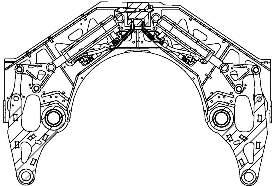
SECTION B-B
